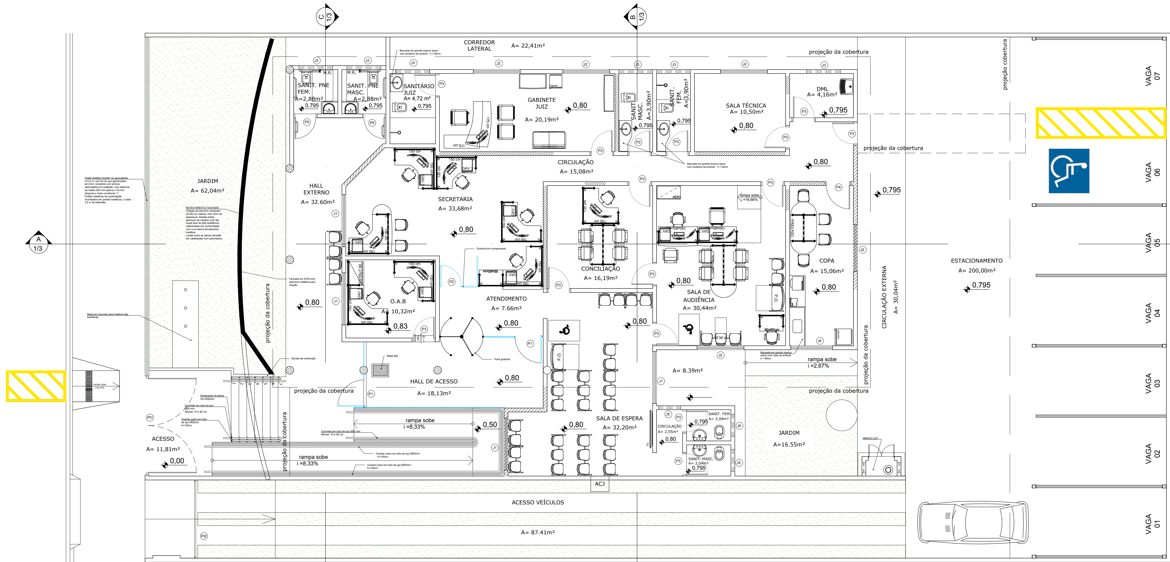
LAYOUT escala 1: 75
